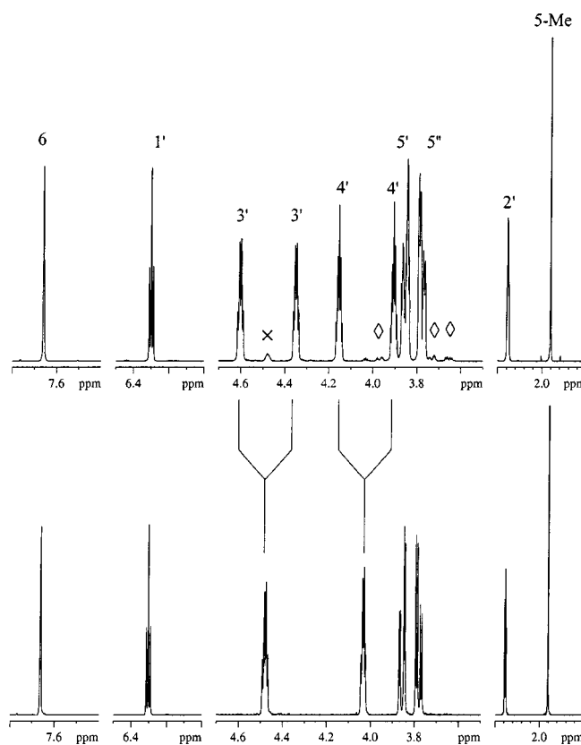
Figure 1. Selected parts of the 1 H-NMR spectrum (600 MHz, D 2 O) of [3,4- 13 C 2 ]thymidine (top) and the same sample measured with 13 C decoupling (bottom); the large splitting of the signals arising from 3'-H and 4'-H (δ = 4.48, respectively) due to an adjacent 13 C atom is indicated, clearly showing high isotope enrichment; a residual signal can be observed in the top spectrum at δ ≈ 4.5 marked with X and occurs as a result of isotope dilution, whereas the intricate pattern (referred to as Δ) s caused by isotope scrambling
