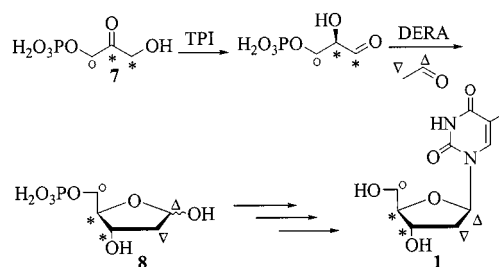
Scheme 1. The key enzymatic aldol condensation of 7 and acetaldehyde yields 8 , which is subsequently converted to 1 ; we have selectively ^{13}\text{C} -labelled the positions marked with an asterisk (*); other positions that may be isotopically substituted are marked with ^\circ or with ^\Delta and ^\nabla .
